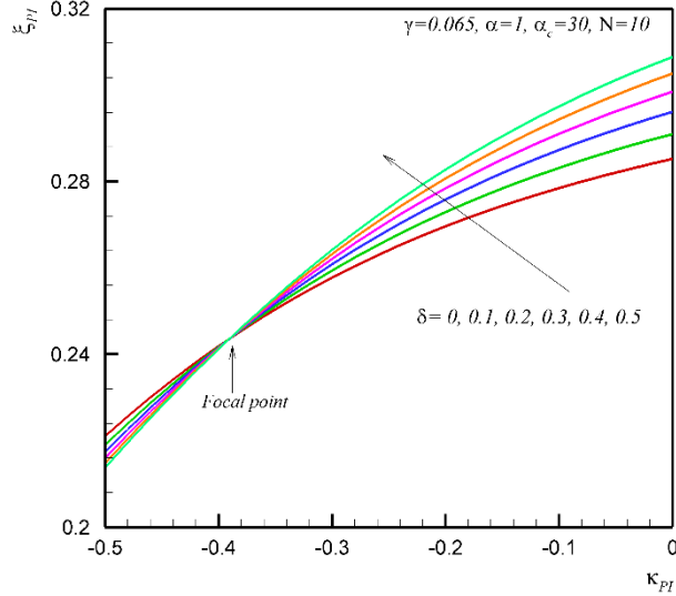
Fig. 7. The pull-in deflection of the nano-actuators as a function of the pull-in dielectric parameter for selected values of the size effect parameter.
